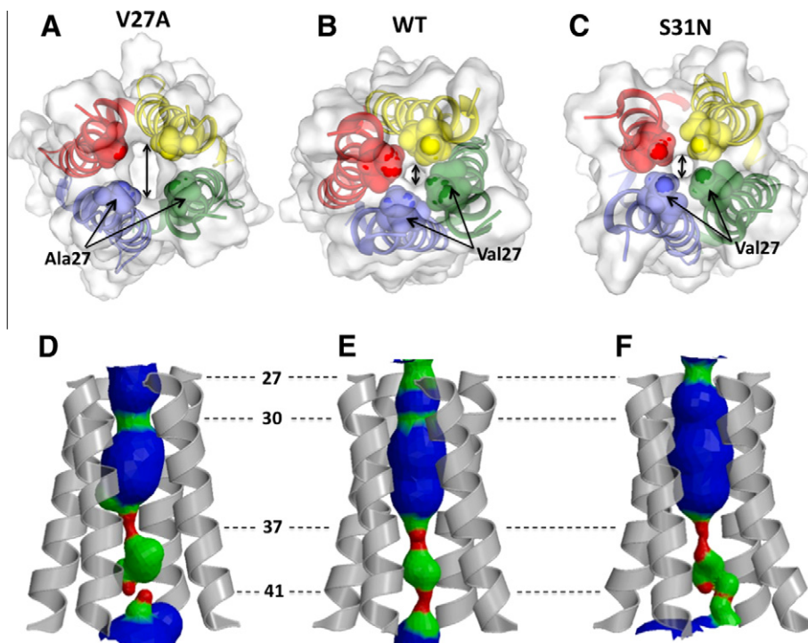
Fig. 3. The size of the channel N-terminal entrance of (A) the V27A mutant (2KWX), (B) WT (2RLF), and (C) the S31N mutant (2KIH) indicated by double headed arrow. The side chains at residue position 27 constrict the channel entrance. Mutating valine at this position to alanine doubles the diameter of the channel opening ( \sim 2.5 Å in WT and the S31N mutant, \sim 5 Å in the V27A mutant). (D–F) The pore surfaces calculated using the program HOLE. (E) The WT structure displays two constrictions in the N terminus at the positions 27 and 30. (D) The V27A mutant displays one constriction at position 30. (F) The S31N mutant is constricted at the position 27, but due to the serine to asparagine substitution at the position 31 the channel forms looser tetramer that results in somewhat larger diameter around Ser30. All of the structures have their C-termini tightly constricted to \sim 1.5 Å by side chains of His37 and Trp41.
